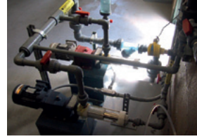
seepex pumps for NaOCl feeding into the discharge line of a vertical turbine pump
